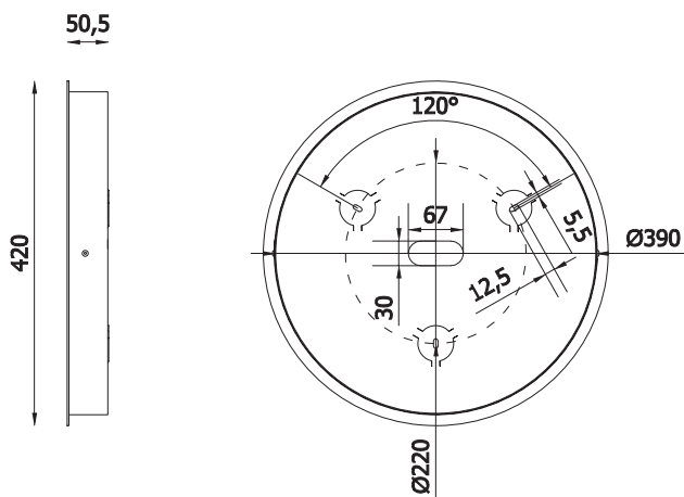
PIASTRA INTERNA / INTERNAL PLATE
